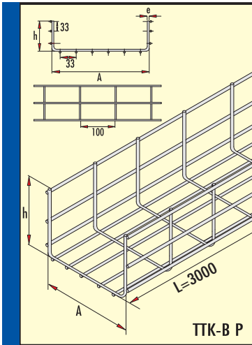
Tel Kablo Kanalı h=85 mm PASLANMAZ TEL (Cr-Ni) Wire-mesh Cable Tray h=85 mm Stainless Steel (Cr-Ni) Проволочный лоток
