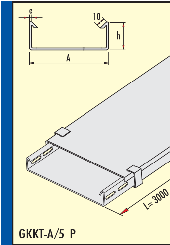
Deliksiz Ağır Hizmet Tipi Kablo Kanalı h=50 mm PASLANMAZ SAC (Cr-Ni) Non Perforated Heavy Duty Cable Trays With Cover h=50 mm Stainless Steel (Cr-Ni) Сверхмощные кабельные лотки с крышкой
