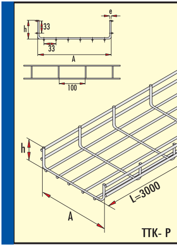
Tel Kablo Kanalı h=50 mm PASLANMAZ TEL (Cr-Ni) Wire-mesh Cable Tray h=50 mm Stainless Steel (Cr-Ni) Проволочный лоток
